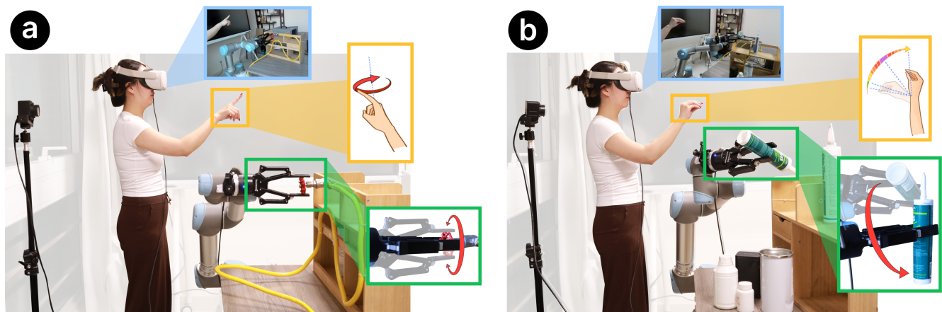
Figure 1: Enhancing robot teleoperation tasks through dexterous finger motion and non-isomorphic rotational gain: (a) gas-leak inspection, where the operator uses FingerCircle to close a valve and WristDNR to inspect potential leak points; and (b) desktop object organization, where the operator uses WristDNR to pick up, align, and place objects onto a shelf.
