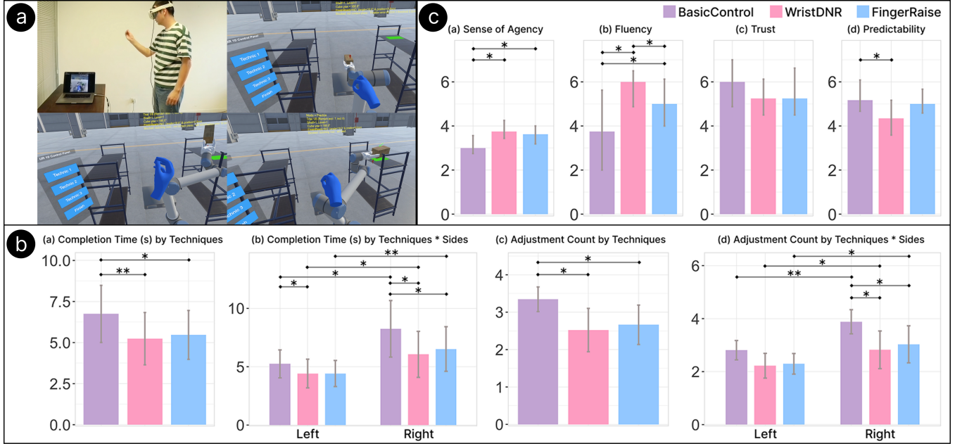
Figure 6: (a) Task 2 setup and interfaces at the beginning, during, and end of a trial; (b) Task 2 results with 95% confidence intervals error bars, and (c) SoA, Fluency, Trust, and Predictability with interquartile range error bars (* p < .05 , ** p < .001 ).
